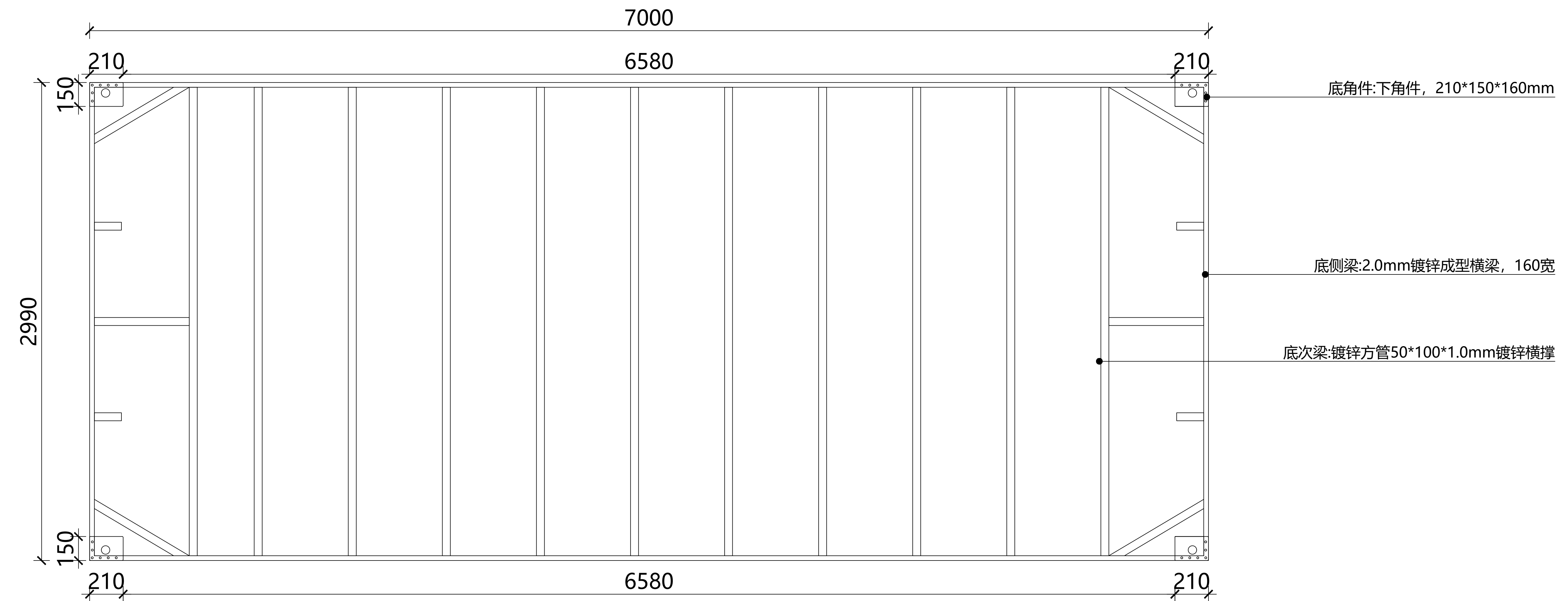
底部框架图Bottom frame drawing
