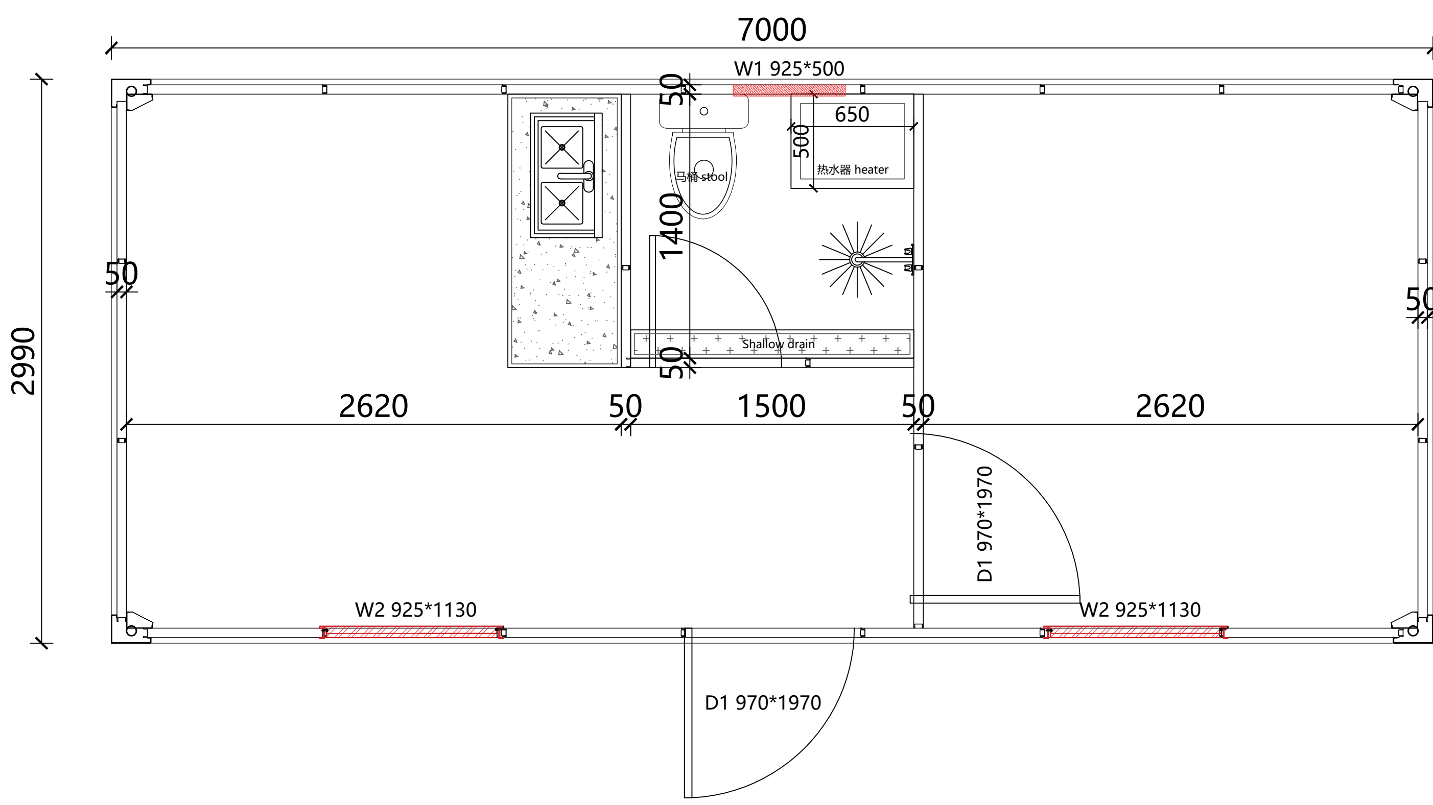
俯视图 vertical view
