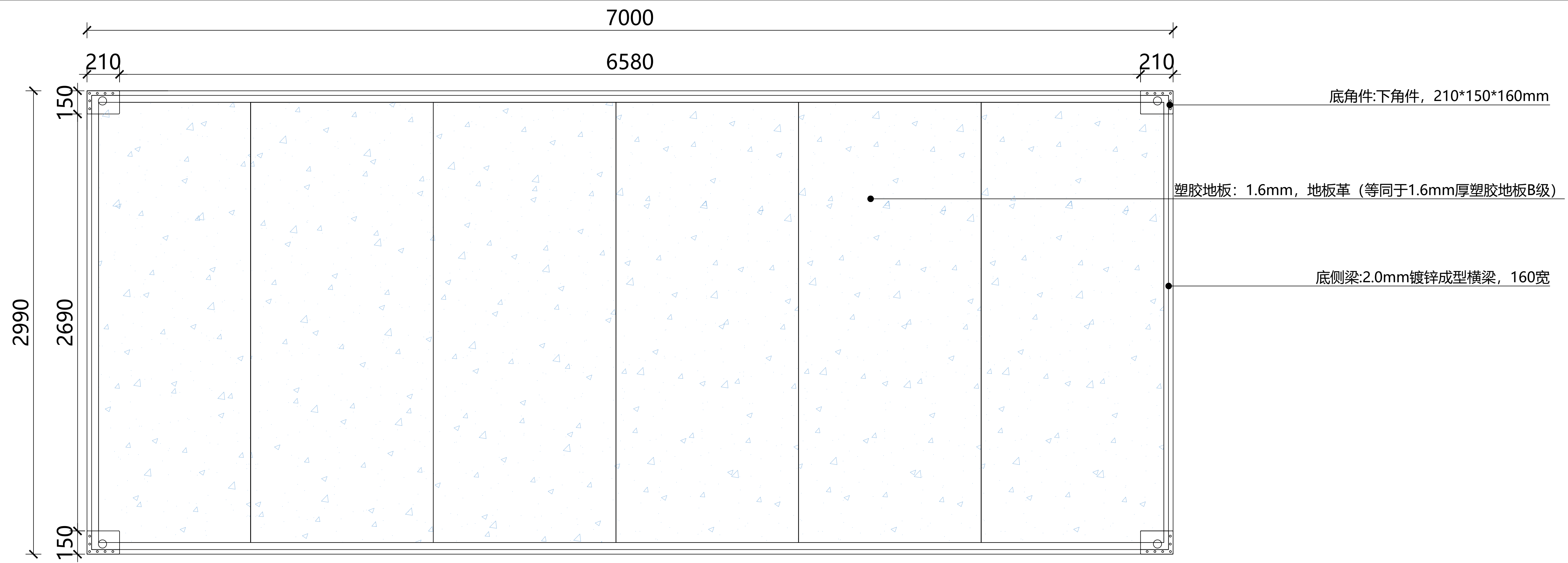
底部框架图Bottom frame drawing
